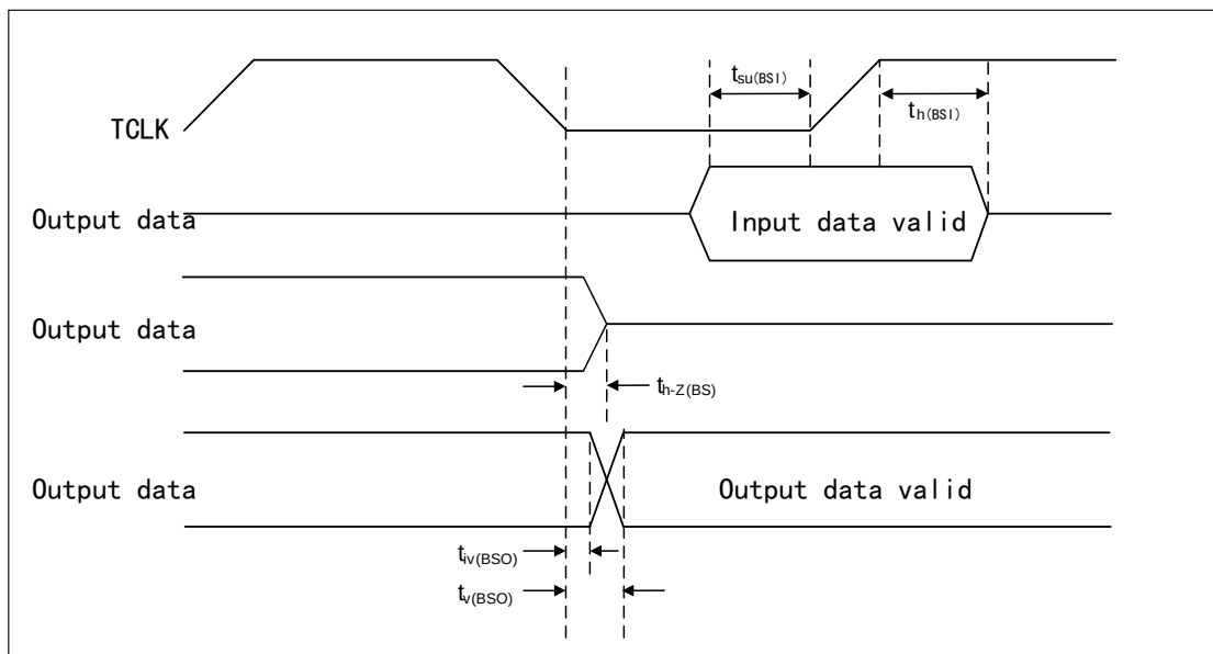
Figure 23 TDO Timing
