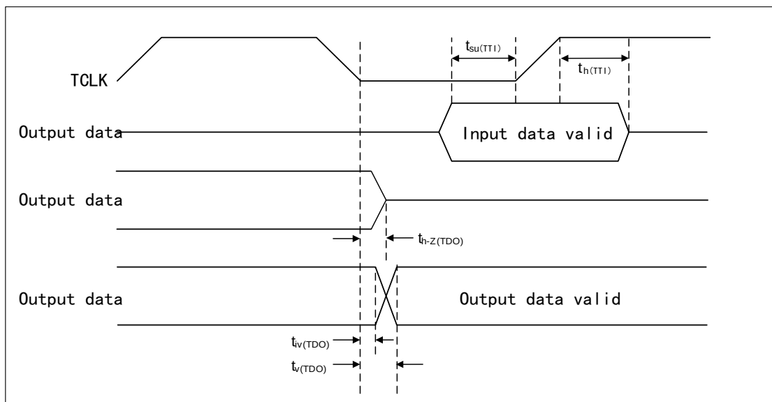
Figure 23 TDO Timing
